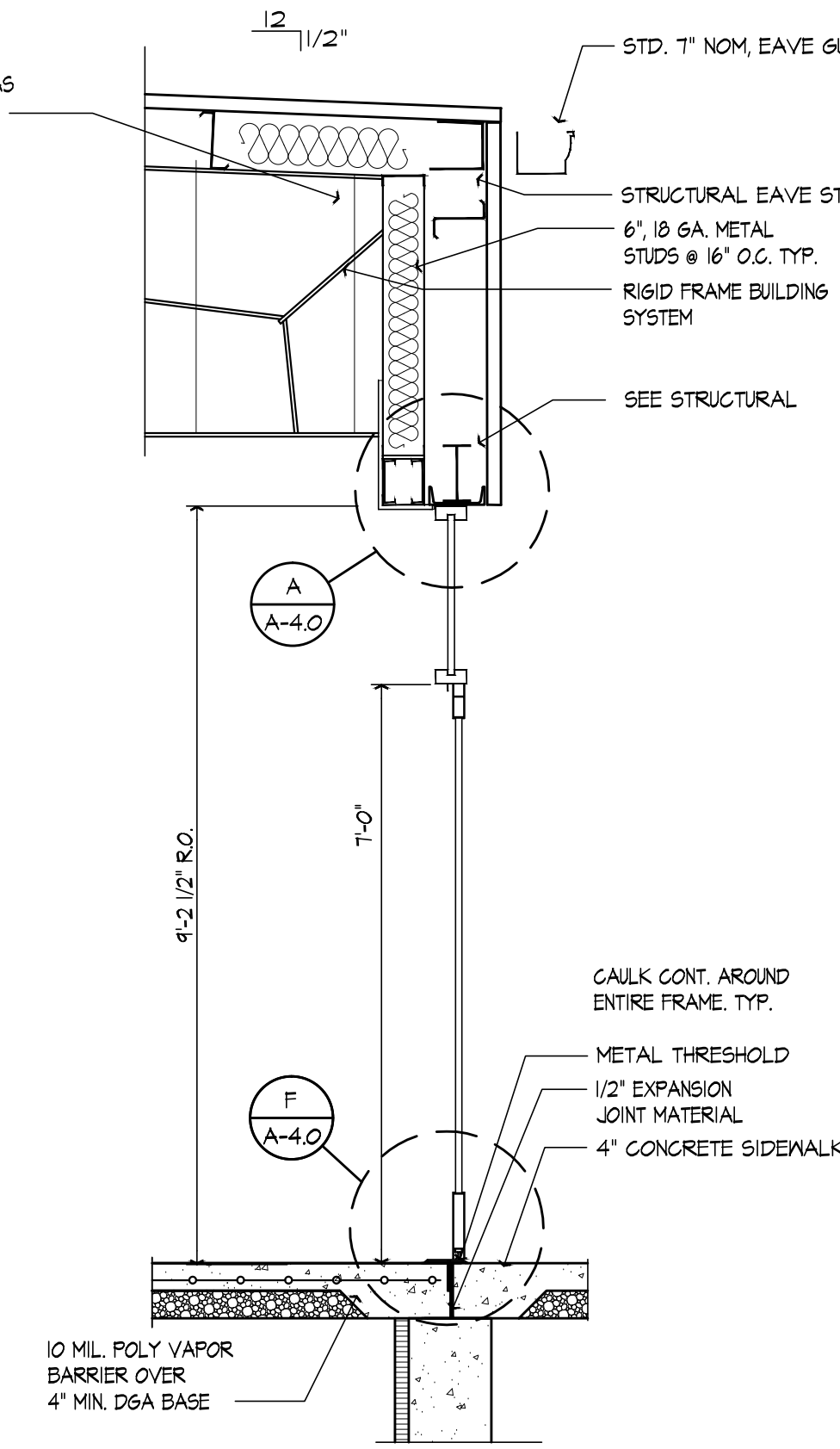
WALL SEC @ ALUM DR. SCALE: 1/2" = 1'-0"
