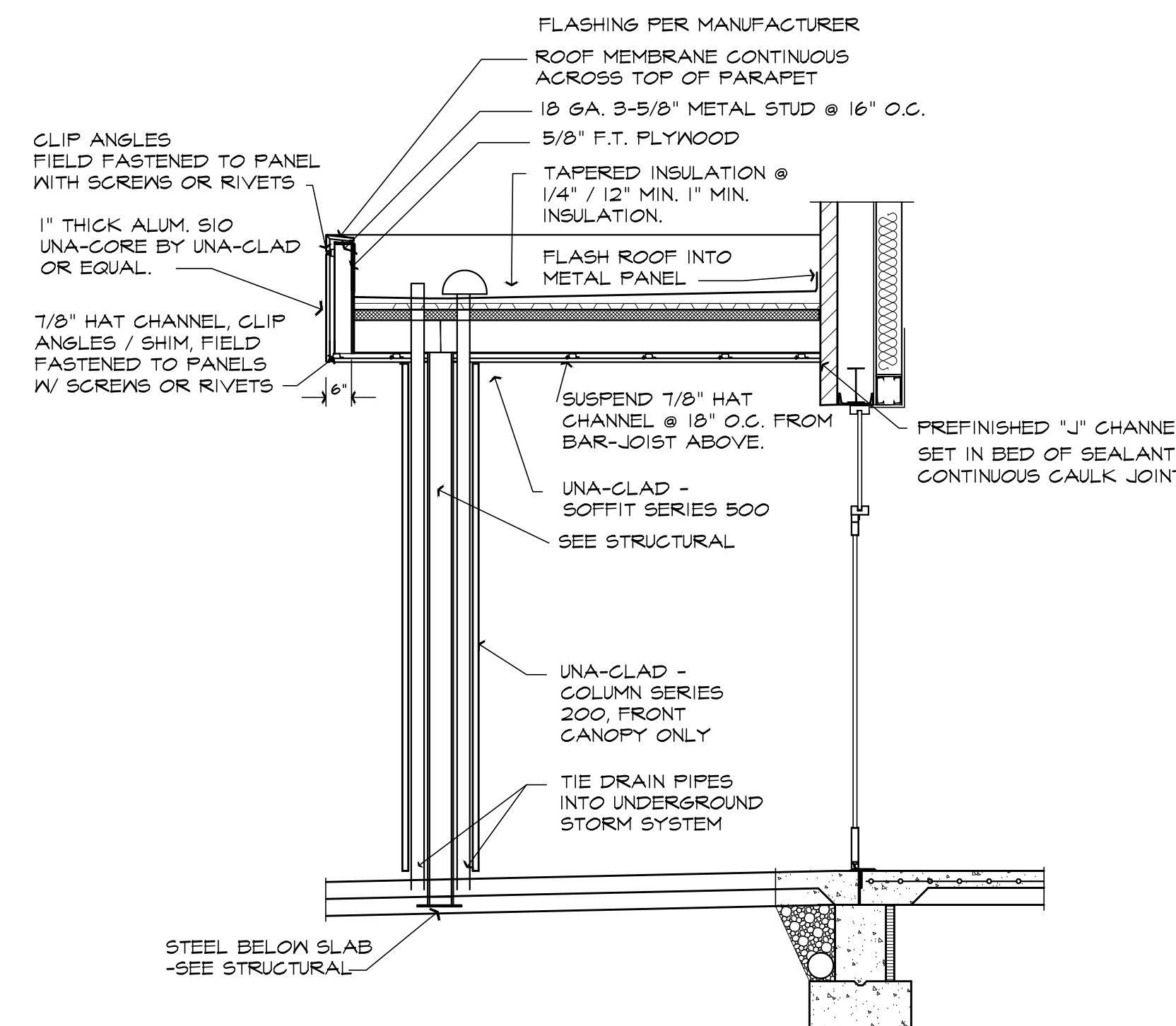
SECTION @ CANOPY SCALE: 3/8" = 1'-0"
