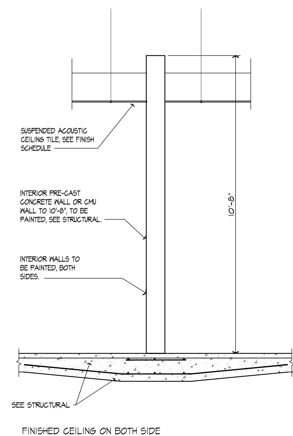
INTERIOR WALL SECTION SCALE: 1/2" = 1'-0"
